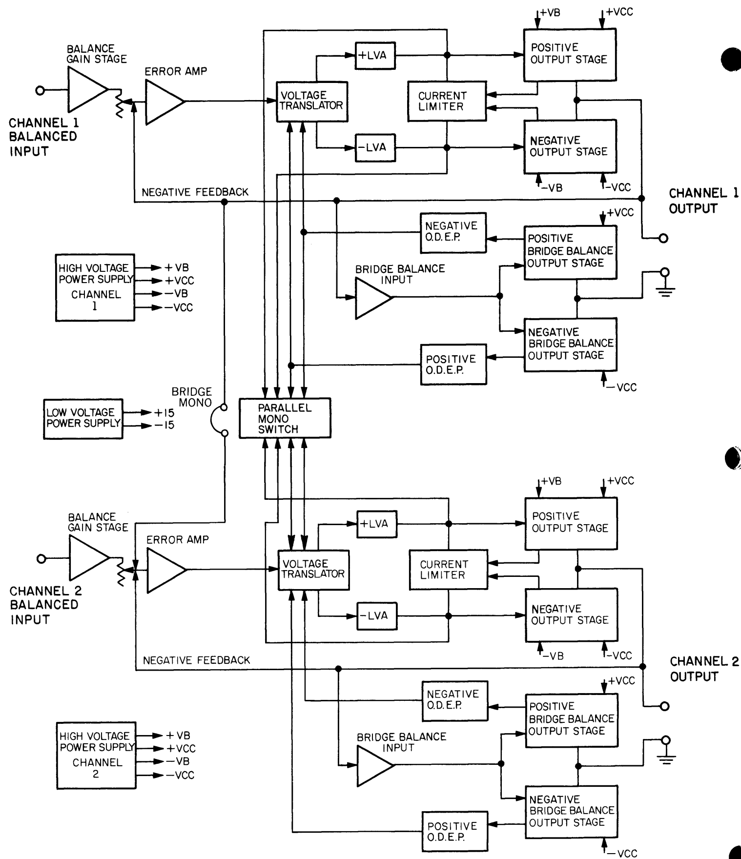
Fig. 4.1 Block Diagram
