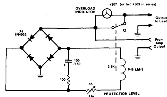
Fig. 3.11 Relay-Controlled Protector with Overload Indicator
