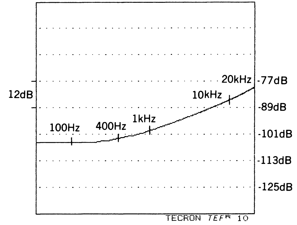
Fig. 2.8 Typical Crosstalk
